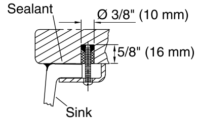
Solid-Surface Installation
