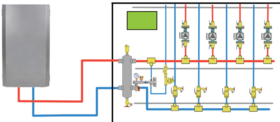
FIGURE 1: Condensing Boiler with Primary/Secondary Piping application:
