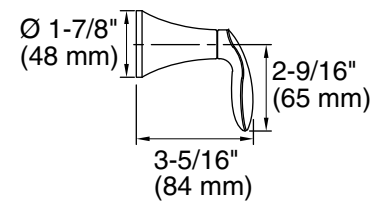
Lever
