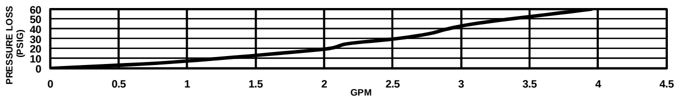
MODEL P6900-TMV-1
