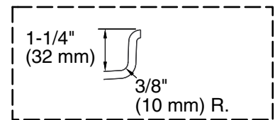
Integral Flange Detail
