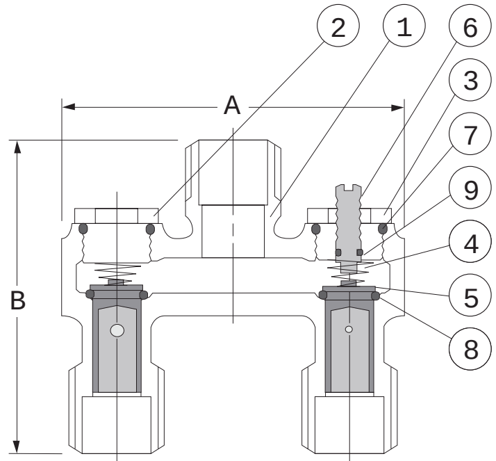
Pictured Model T-20A Cut-away
