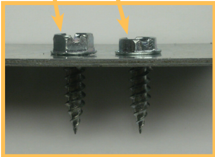
High Head Saber Screw vs. standard screw
