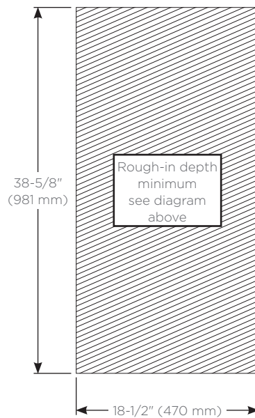
Rough-in Dimensions
