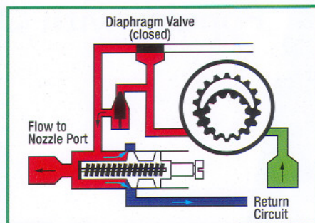
Conventional Pump — full speed
