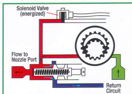
CleanCut Pump — valve energized
