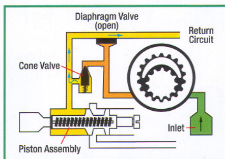
Conventional Pump — start-up
