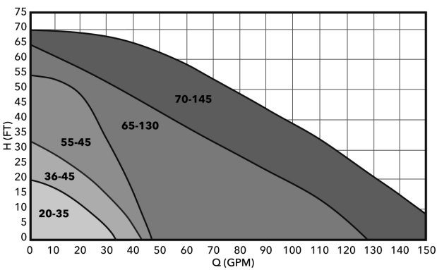
ecocirc XL High Head Performance Range
