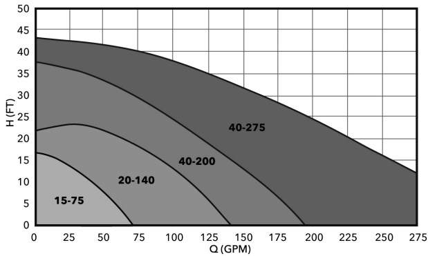
ecocirc XL High Flow Performance Range
