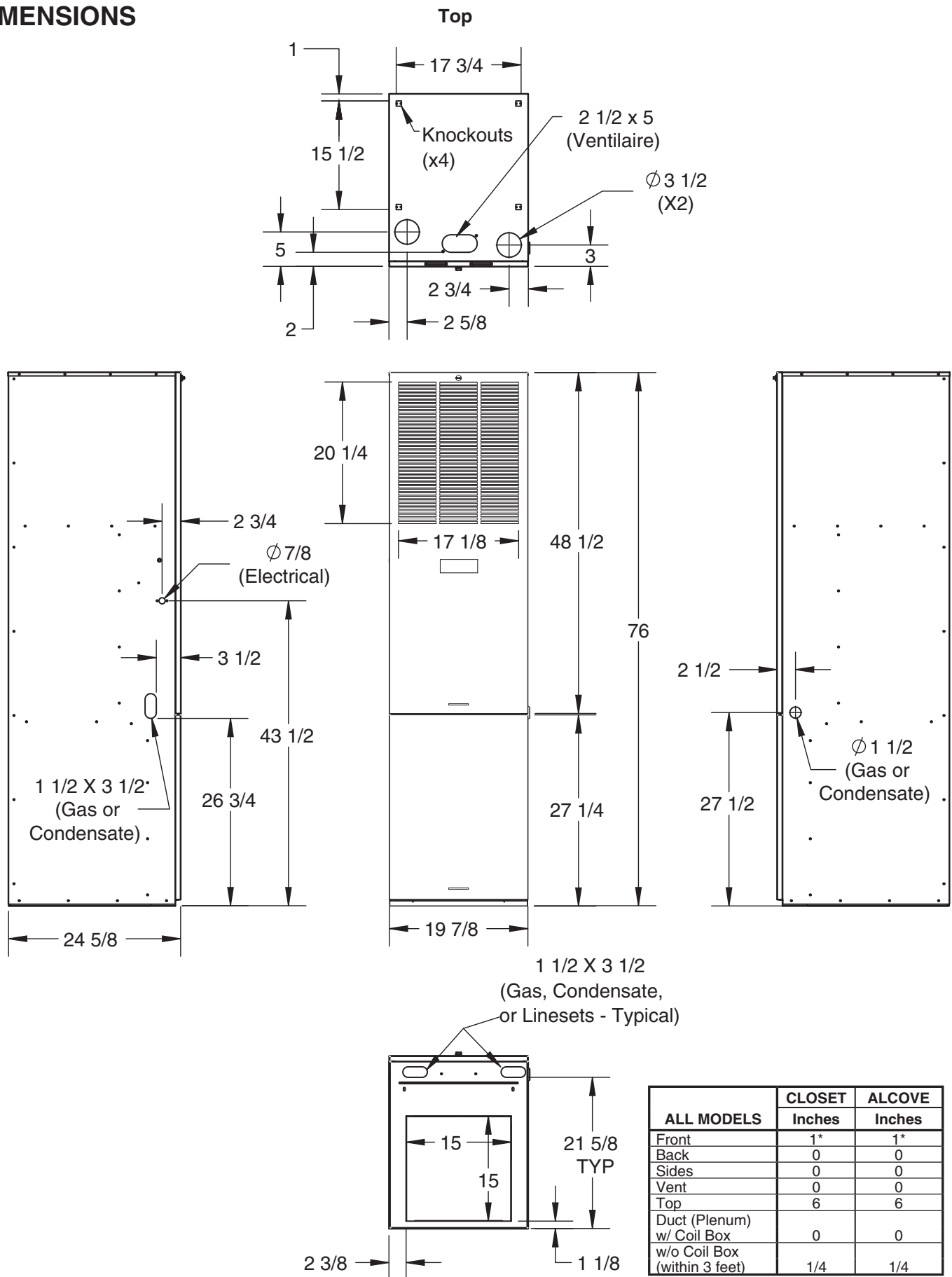
Minimum Clearances
