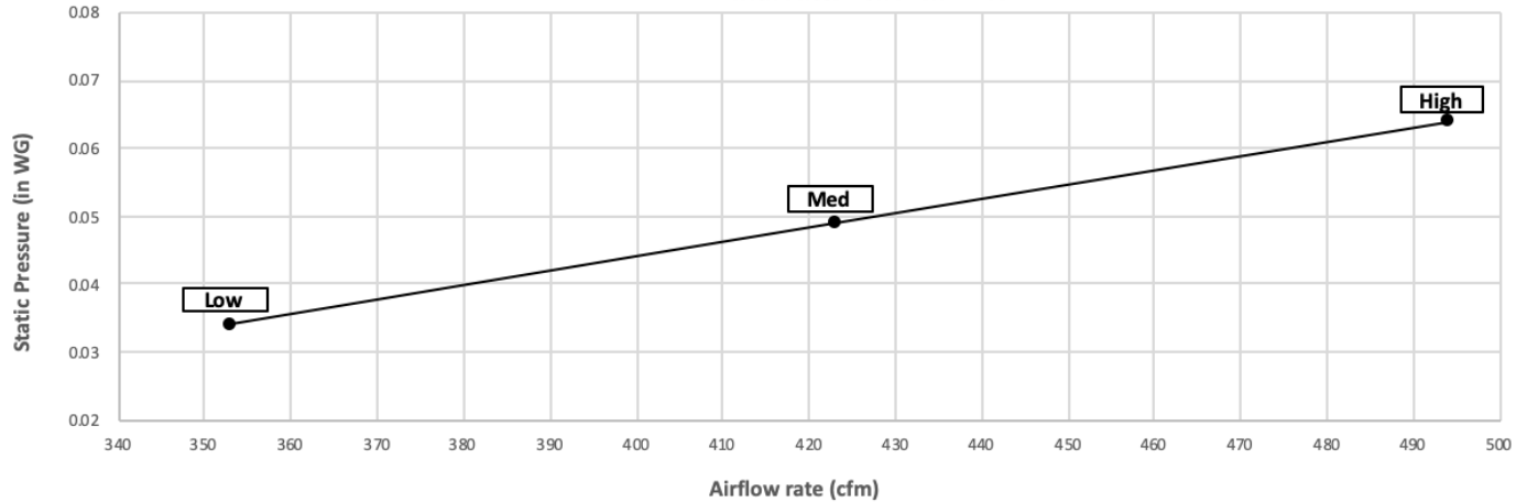
PEAD-A12AA7 with Filter Box FBM2-2-A
