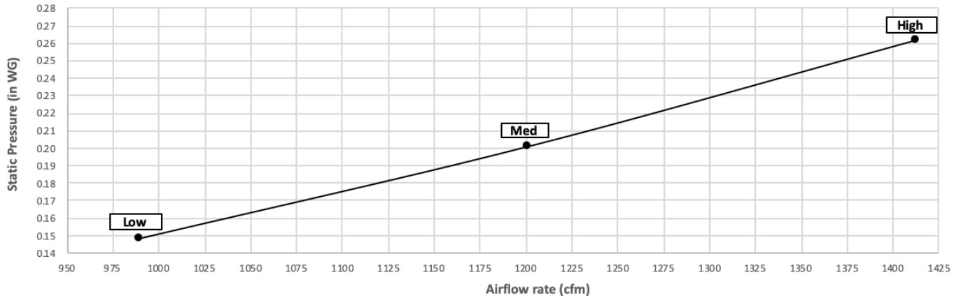
PEFY-P48-NAMU-E3 with Filter Box FBM2-4-A
