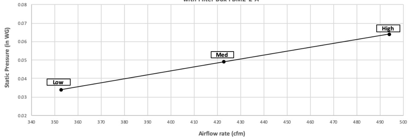
PEFY-P15-NAMU-E3 with Filter Box FBM2-2-A
