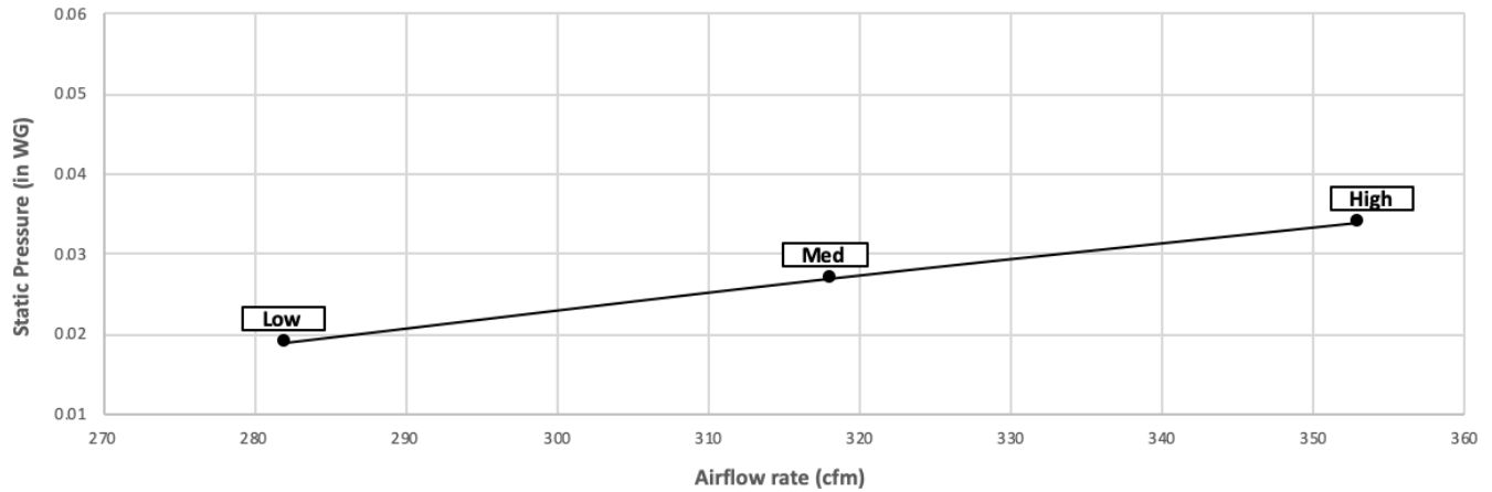
PEAD-A09AA7 with Filter Box FBM2-2-A
