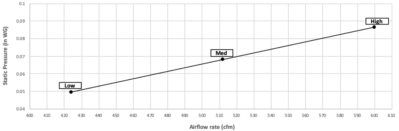
PEFY-P18-NAMU-E3 with Filter Box FBM2-2-A
