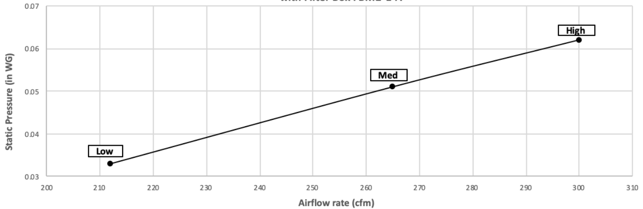
PEFY-P06/P08-NAMU-E3 with Filter Box FBM2-1-A
