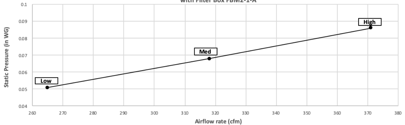
PEFY-P12-NAMU-E3 with Filter Box FBM2-1-A
