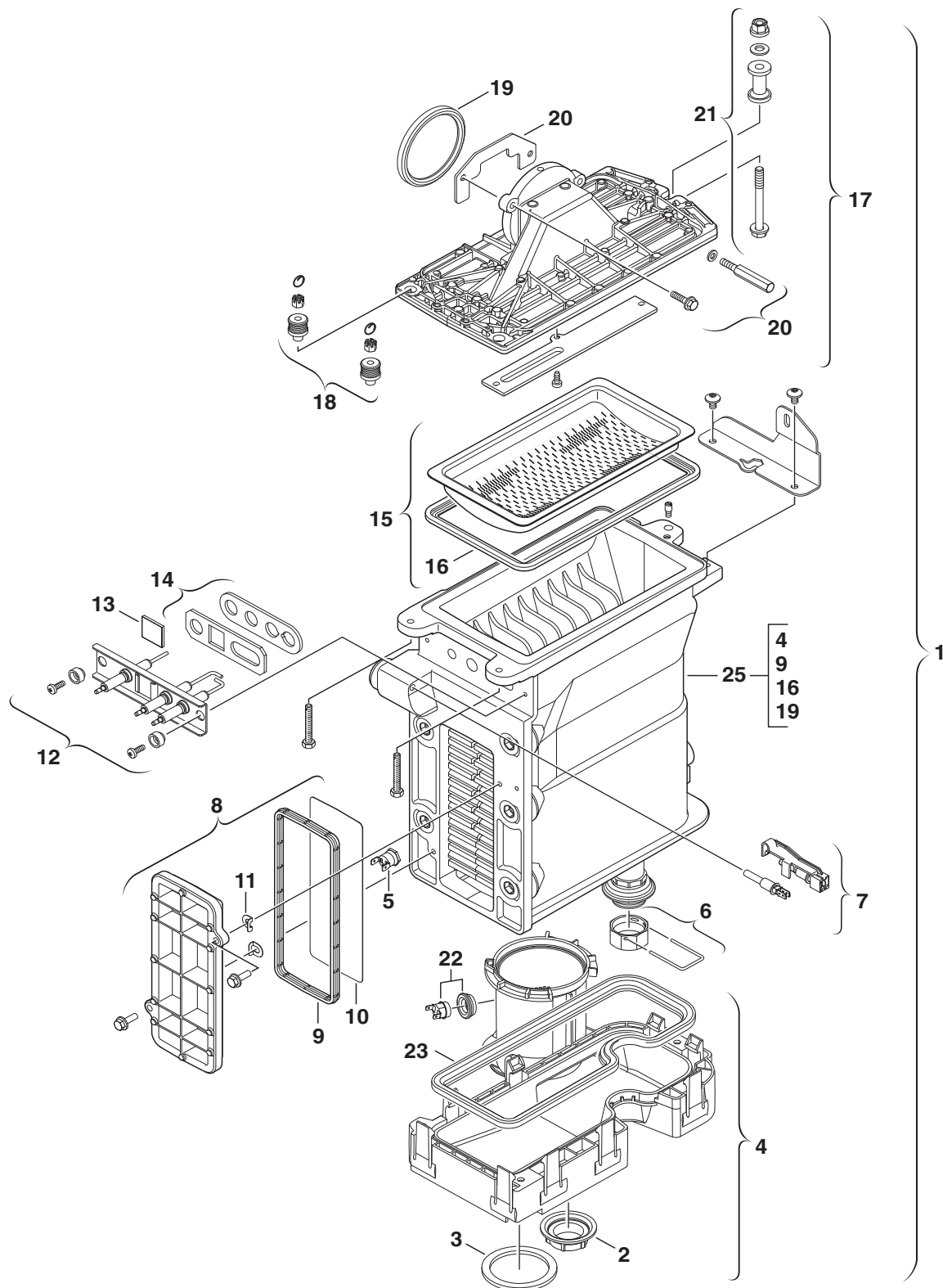
Fig. 94 Group 2 - Burner/Heat exchanger Greenstar
