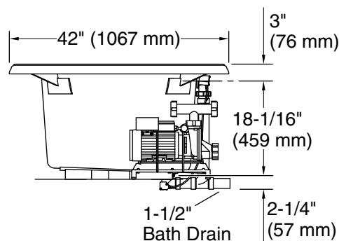
Blower Control Access 34" (864 mm) W x 15" (381 mm) H
