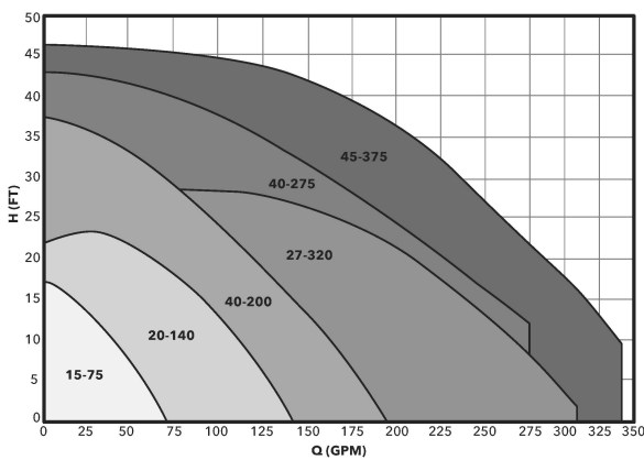
ecocirc XL High Flow Performance Range Curve
