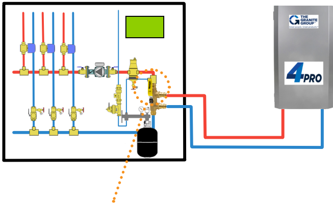
Primary / Secondary Piping Pro-Pal Loop Purge Tee OPEN
