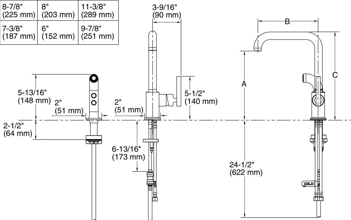
Product Diagram
