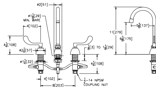
Note: All dimensions are for reference only. Do not use for pre-plumbing
