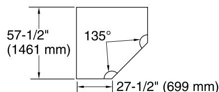
Drop-In Rim Style Cut-Out Detail
