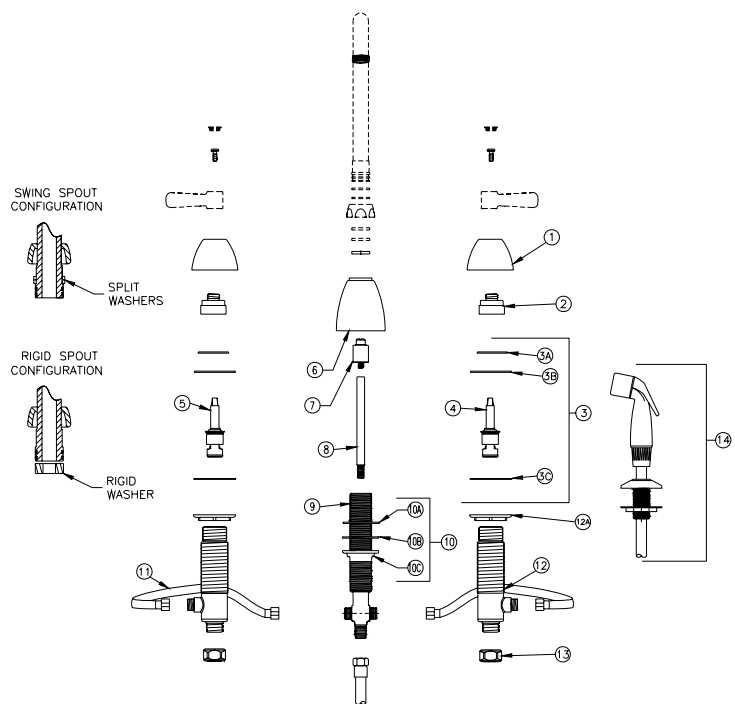
Z831A1-XL-HS PICTURED
