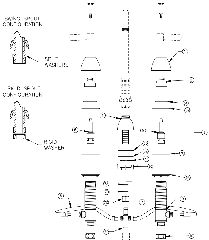
Z831A1-XL PICTURED
