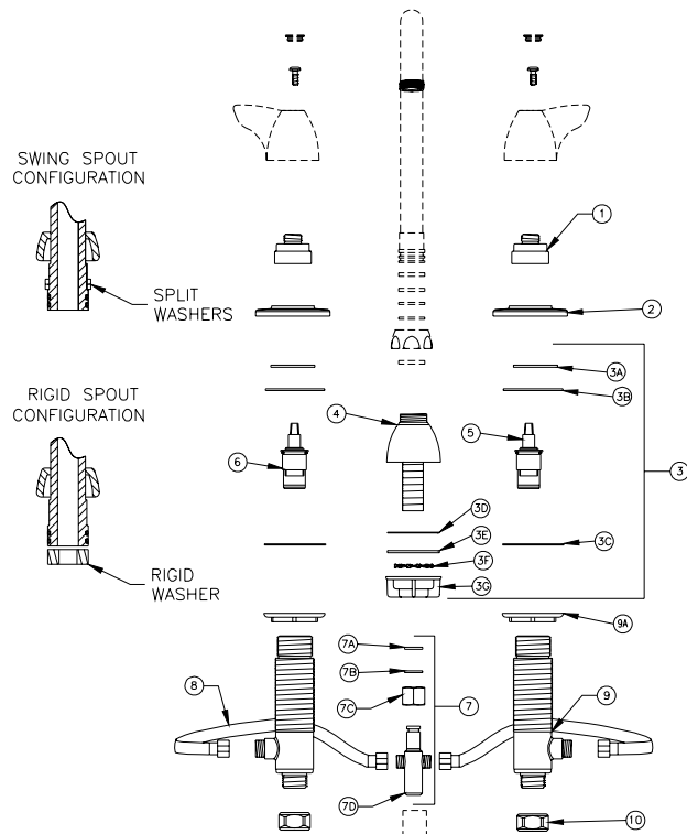
Z831A1-XL-HS PICTURED
