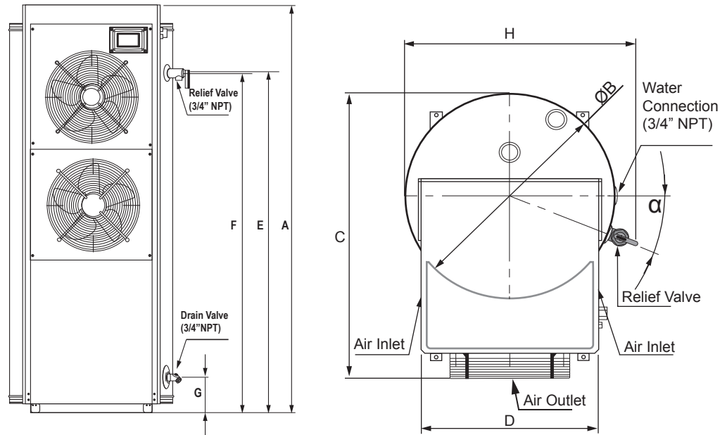
Figure 1. Rough-In Dimensions
