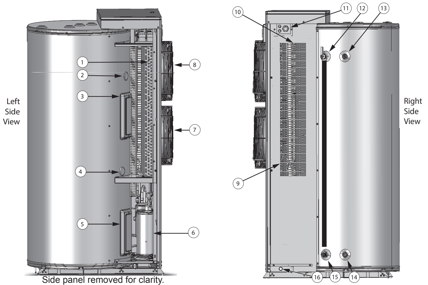
Figure 3. Left and Right Side Views
