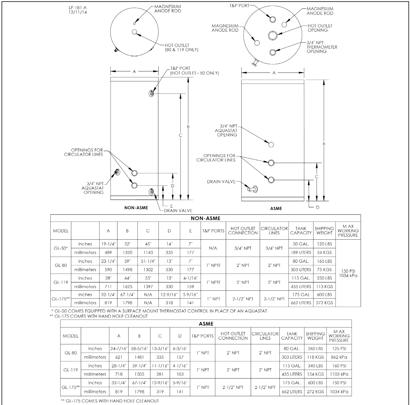
Figure 2 - Specifications and Dimensions - NOTE: A drain valve port IS NOT included on GL-50 models.
