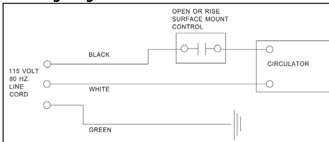
Figure 4 - Wiring the Control
