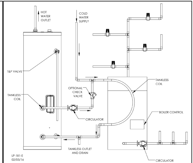
Figure 5 - Typical Storage Tank Installation - All Other Models
