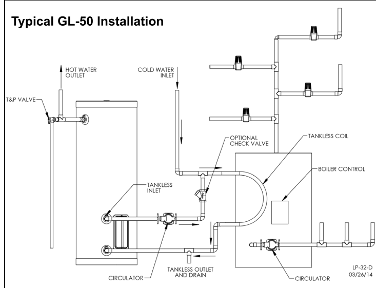
Figure 3 - Typical GL-50 Installation
