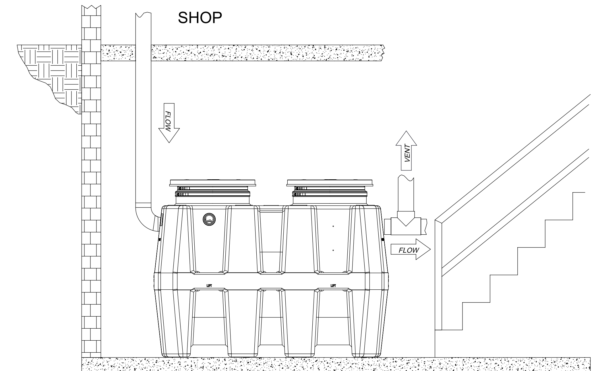
ON-THE-FLOOR DETAIL
