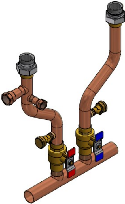
Closely Spaced Tee
