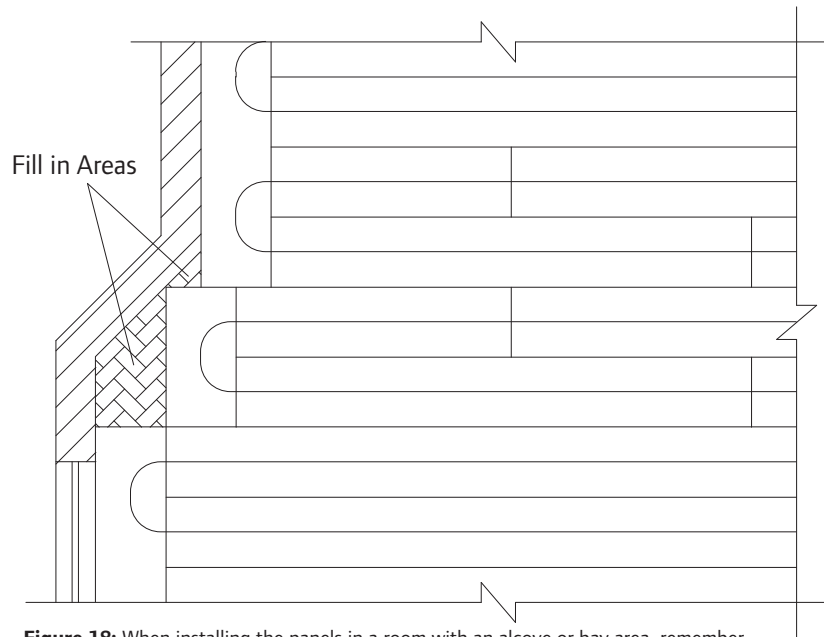
Figure 18: When installing the panels in a room with an alcove or bay area, remember to allow enough room for the Return Trak panels. Fill any areas not covered with panels with \frac{1}{2} " plywood.
