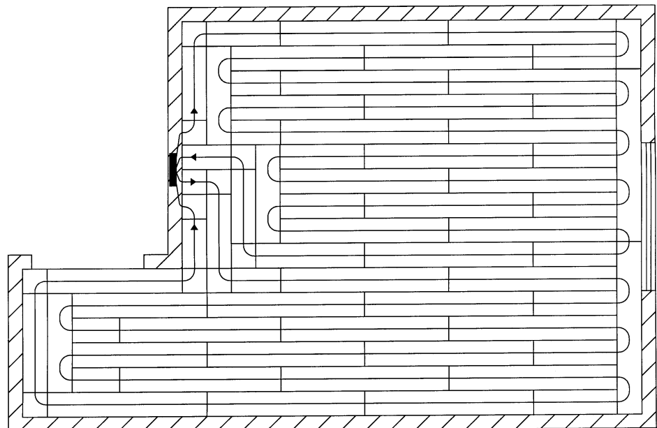
Figure 6: Manifold Location in the Wall
