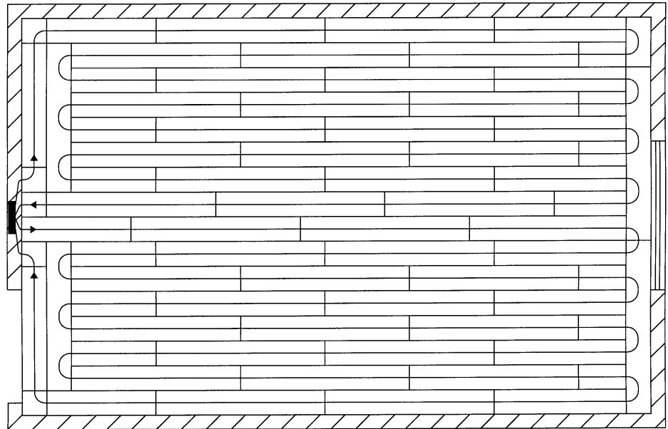
Figure 5: Manifold Location in the Wall
