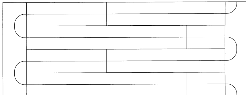
Figure 16: Correct Panel Placement for Serpentine Pattern
