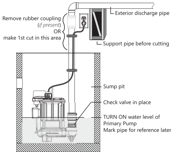
Figure 3. Mark and Cut Pipe
