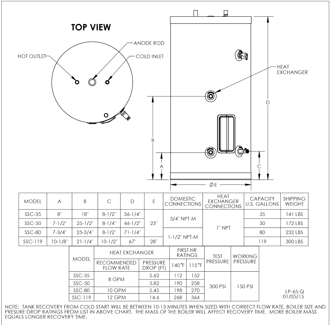
Figure 2 - Dimensions
