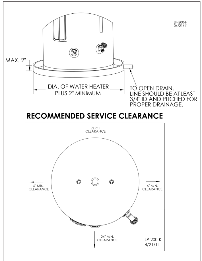
Figure 1 - Drain Pan Installation and Recommended Service Clearances
