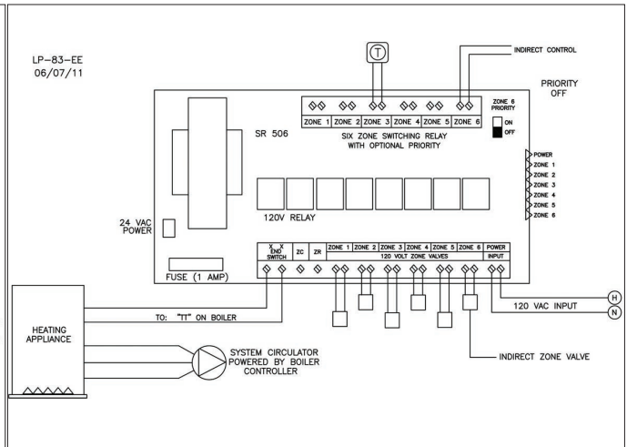
Figure 10 - Wiring with Zone Valves
