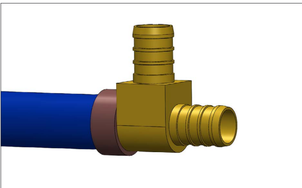
Ring not placed over sealing barbs of fitting. Ring too far forward or too far back & not fully over sealing barbs.
