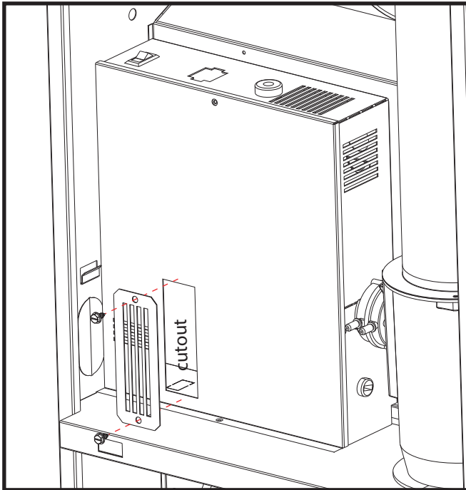
Figure 3. Vent Plate for Control Cover
