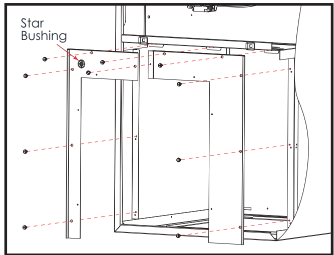
Figure 4. Coil Close Off Panels
