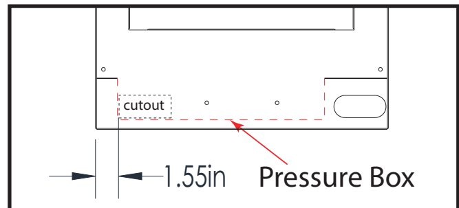
Figure 5. Bottom Pan Modification (Top View)
