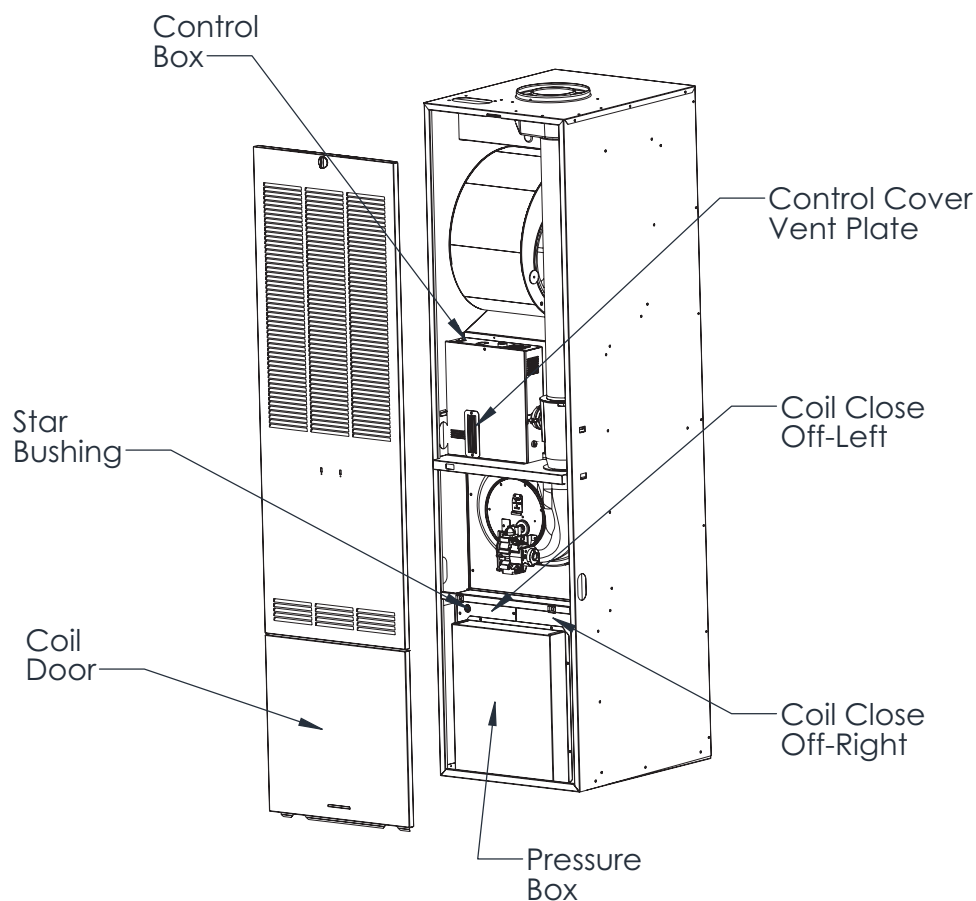
Figure 1. MG1E "B" Cabinet Part List
