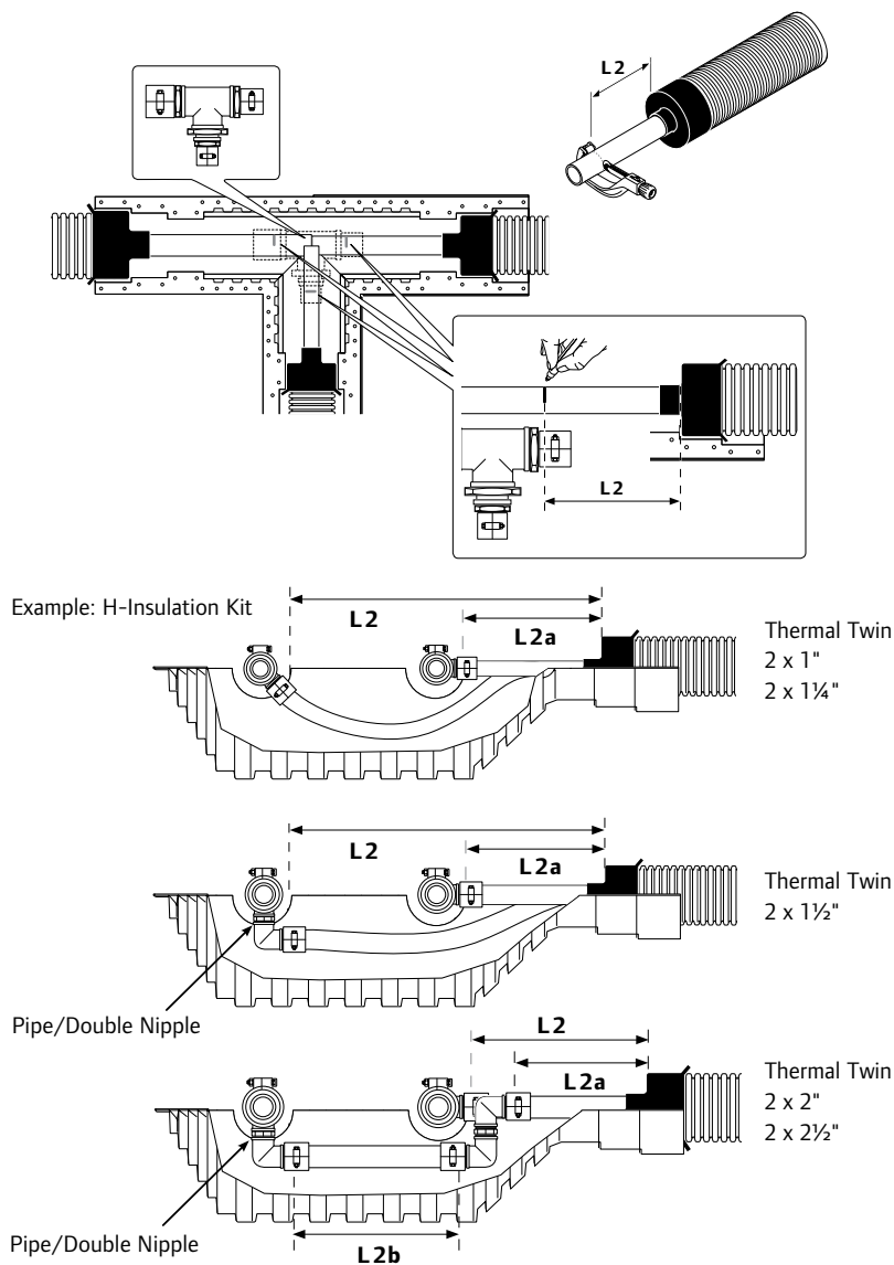
Figure 4-47: Determining Lengths for Assembly and Pipe Styles
