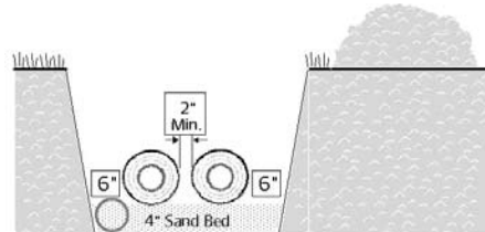
Figure 4-6: Trench Preparation
