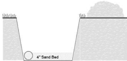
Figure 4-5: Trench Preparation
