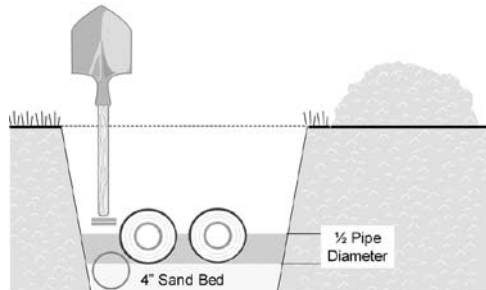
Figure 4-7: Trench Preparation
