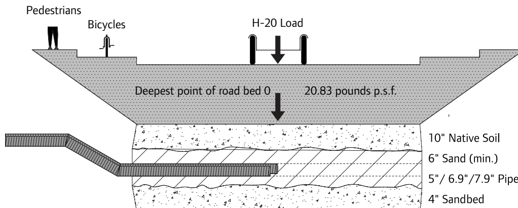
Figure 4-10: Traffic Load
