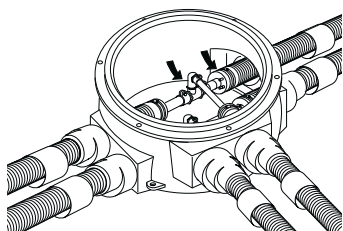
Figure 4-39: Final Connections
