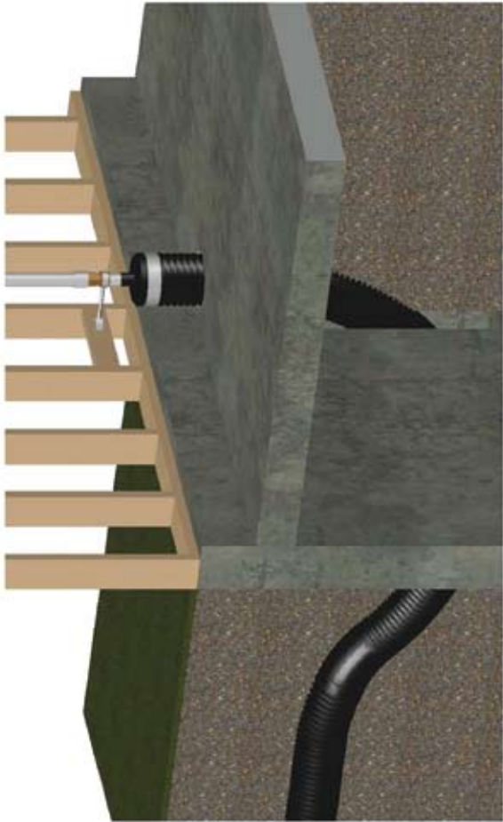
Slab-on-grade Installation
