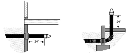
Figure 4-12: Allow 24" of Extra Pipe at Ends
