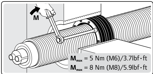
Figure 4-74: Tighten to Maximum Torque
