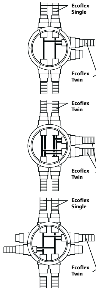
Figure 3-7: Pipe Connection Example
