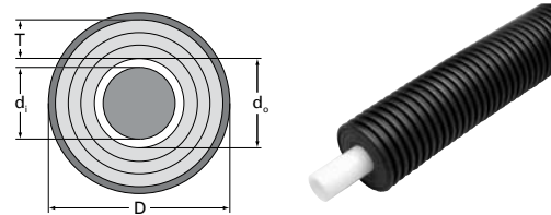
Figure 2-4: Ecoflex Thermal Single Piping
