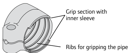
Figure 4-23: Eccentric Design of the WIPEX Fitting
