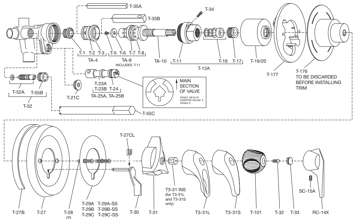
FIGURE 9 Parts Breakdown
