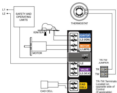
Figure 7 – 7505A (for replacement of R7184A)
