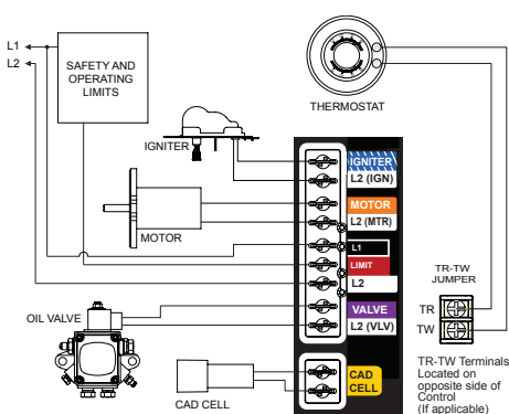
Figure 9 – 7505P (for replacement of R7184P)
