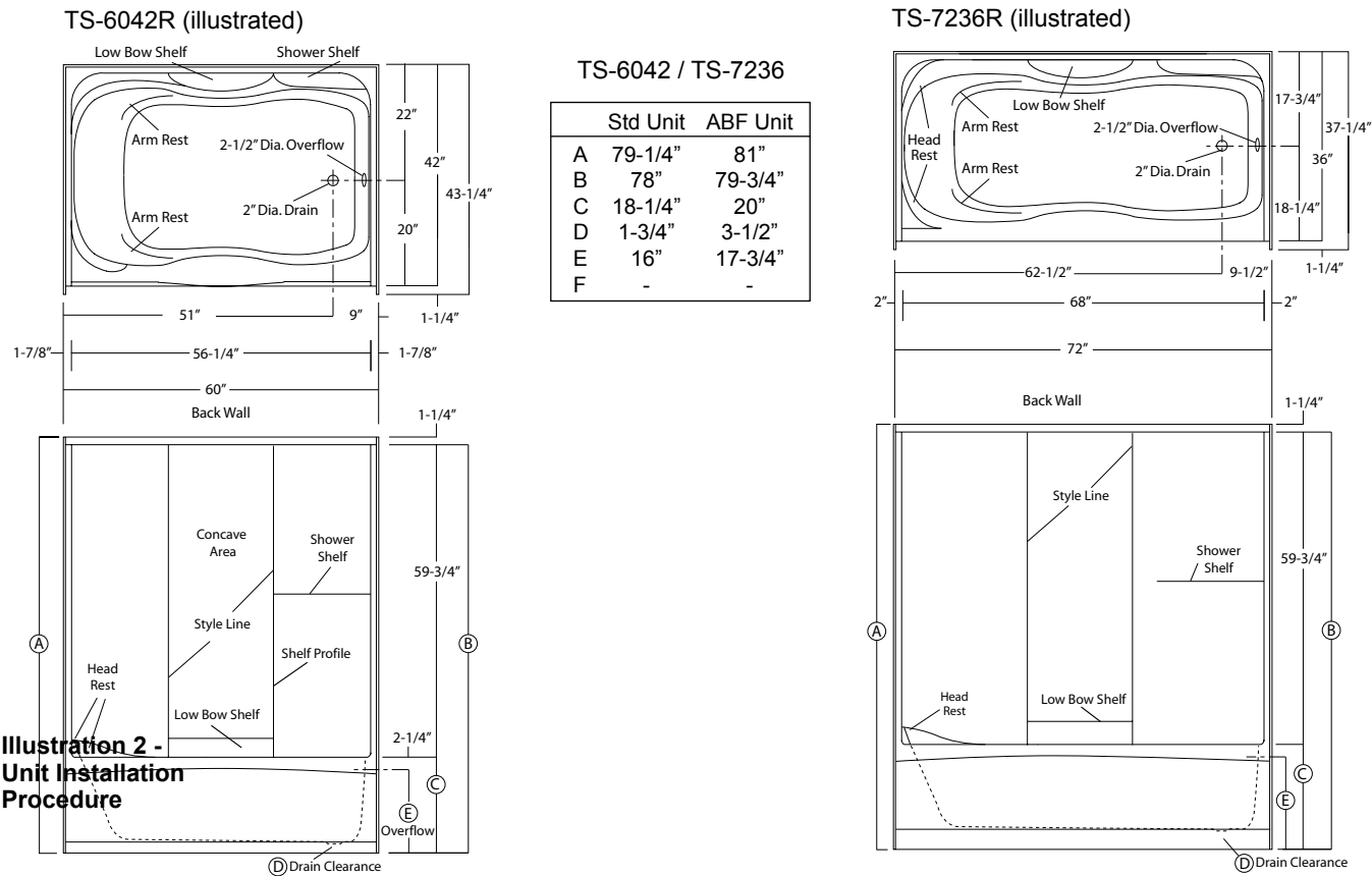
Illustration 1c - End Drain, Unit Dimension & Alcove Framing Guidelines (dimensional tolerance + / -1/8")
