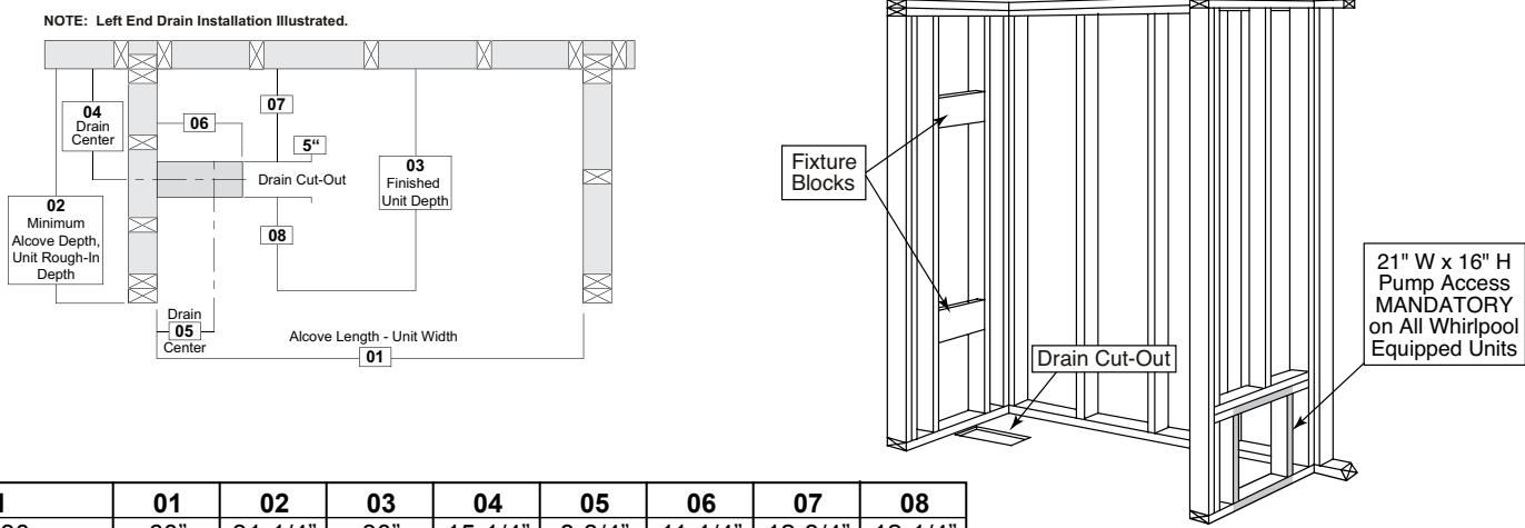
Illustration 1c - End Drain, Unit Dimension & Alcove Framing Guidelines (dimensional tolerance + / -1/8")
