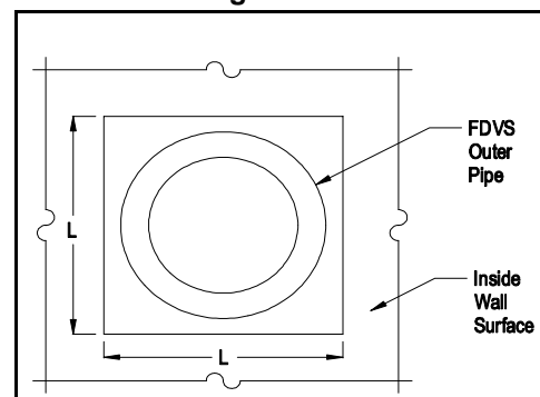
Figure 1 – End View
