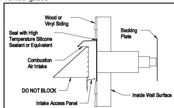
Figure 2 – Side View
