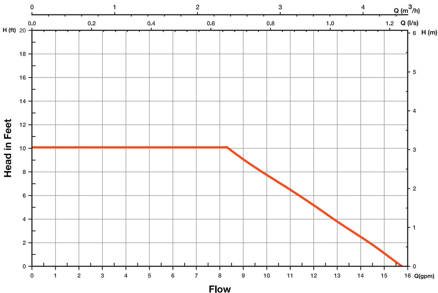
007e™ Performance Curve
