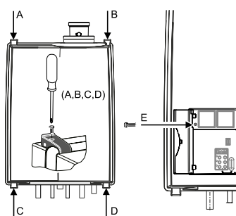
Removing casing
