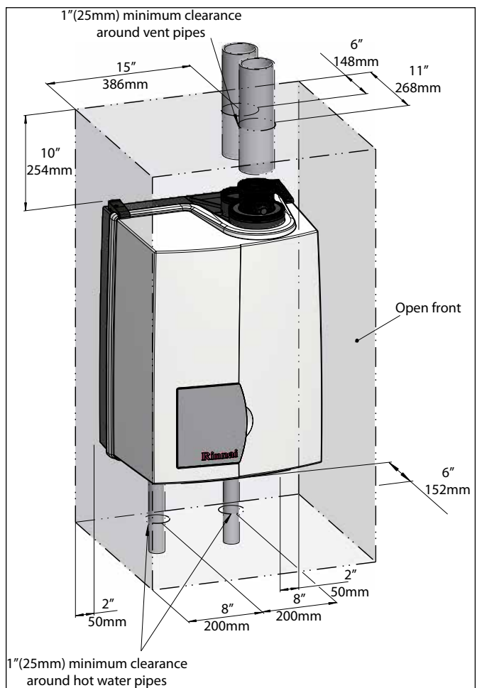
Alcove installation
