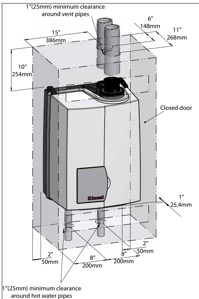
Closet installation
