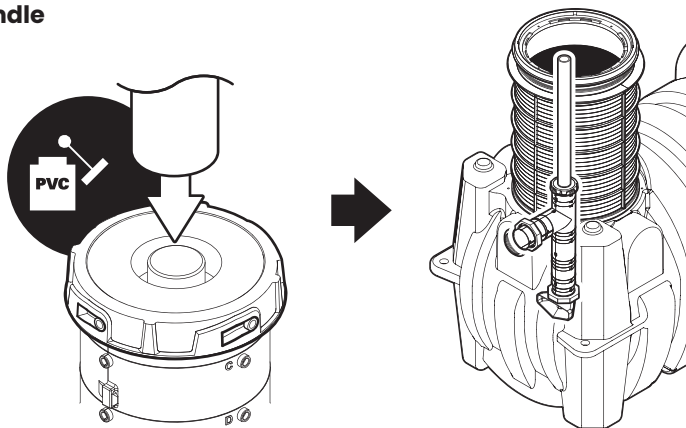
Finished installation showing optional extension handle
