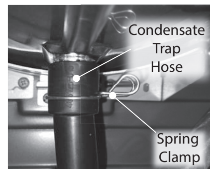
Figure 259 - Spring Clamp, Condensate Hose
