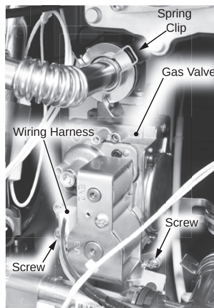
Figure 77 - Gas valve location and connections
