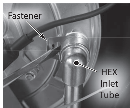
Figure 133 - Remove fastener securing HEX inlet tube
