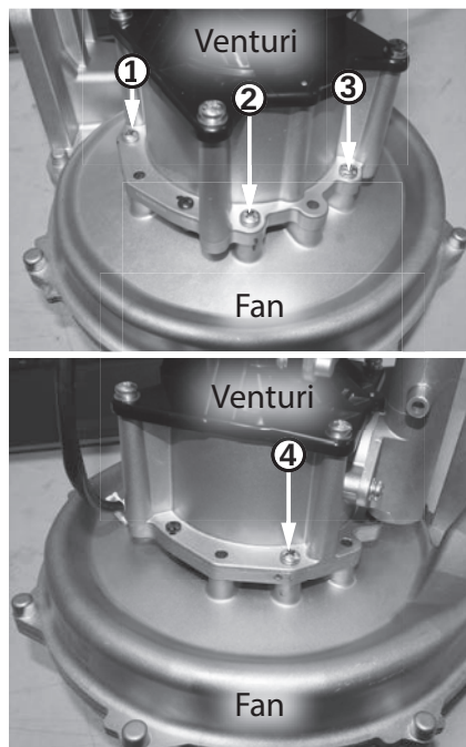
Figure 100 - Locate venturi and fan screws
