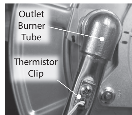
Figure 260 - Thermistor Clip, Outlet Burner Tube
