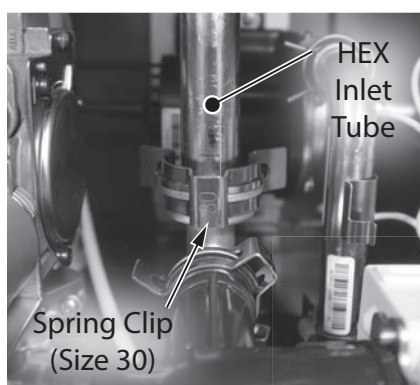
Figure 188 - Remove spring clip securing HEX inlet tube
