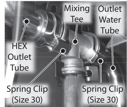
Figure 200 - Remove spring clips from HEX outlet tube and outlet water tube
