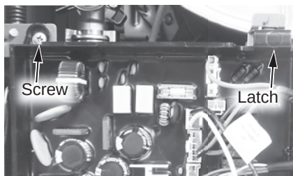
Figure 212 - Control board location
