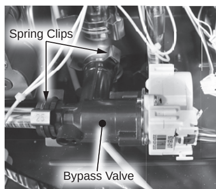
Figure 175 - Bypass valve location
