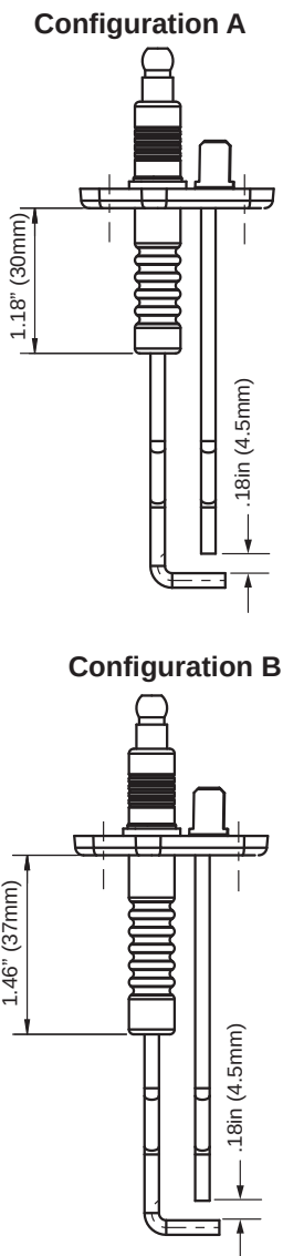
Figure 3: Ignitor rod configurations
