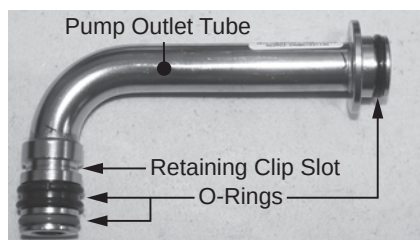
Figure 181 - Pump outlet tube O-rings
