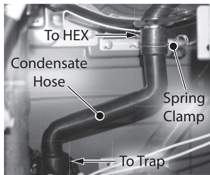
Figure 130 - Disconnect condensate hose
