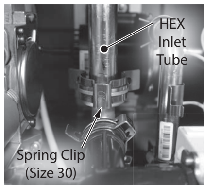
Figure 132 - Remove spring clip securing HEX inlet tube
