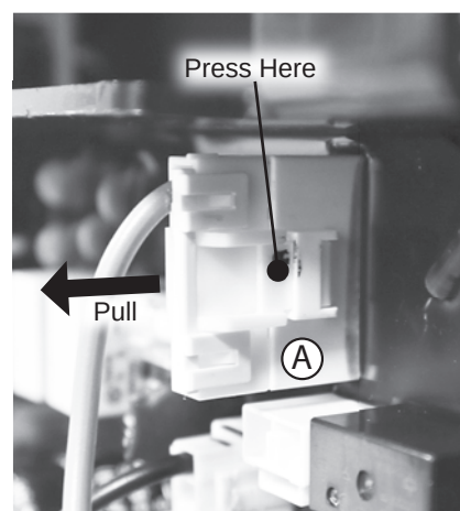
Figure 55 - Wiring harness A removal.
