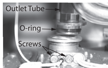
Figure 228 - O-ring location
