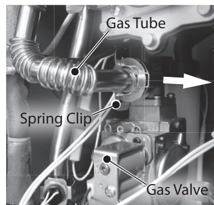
Figure 128 - Remove gas tube spring clip
