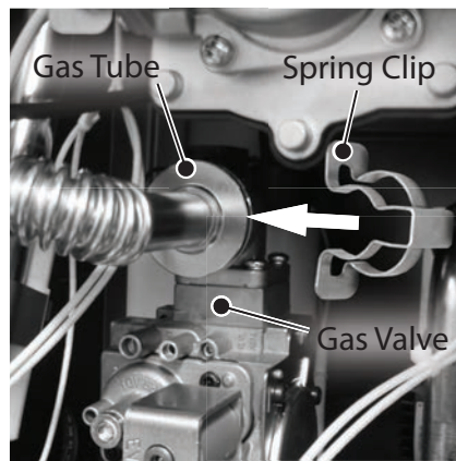
Figure 90 - Secure gas tube with spring clip
