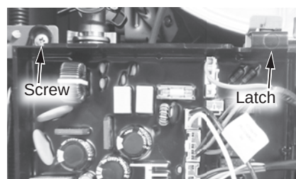
Figure 36 - Control board location
