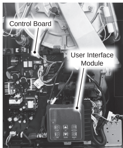
Figure 13 - User Interface Module
