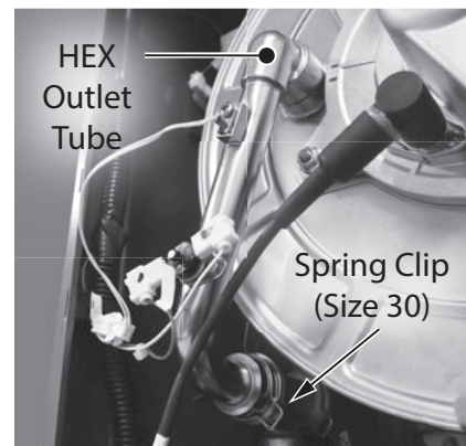
Figure 134 - Remove spring clip securing HEX outlet tube
