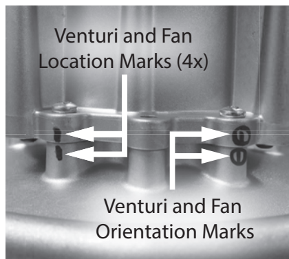
Figure 101 - Screw hole and orientation markings
