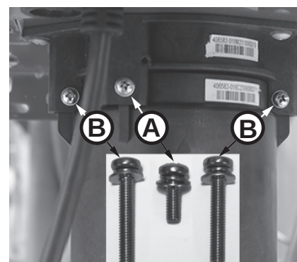
Figure 216 - Identify cartridge screws
