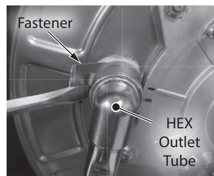
Figure 135 - Remove fastener securing HEX outlet tube
