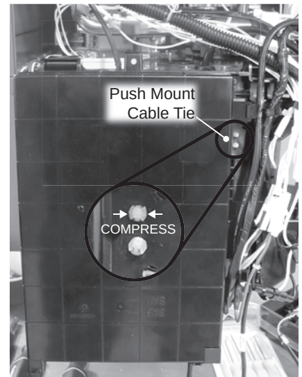
Figure 45 - Locating the push mount connector
