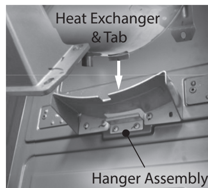
Figure 150 - Insert tab into hanger
