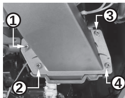
Figure 129 - Remove fan assembly screws
