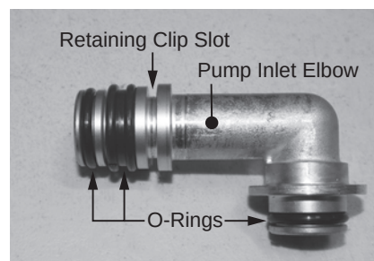
Figure 179 - Pump inlet elbow O-rings
