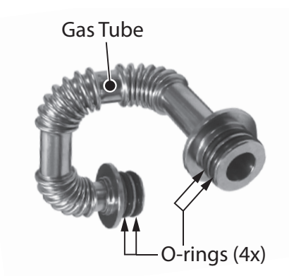
Figure 95 - Install O-rings to gas tube
