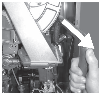
Figure 191 - Remove HEX inlet tube
