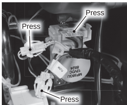
Figure 213 - Locating wiring harnesses
