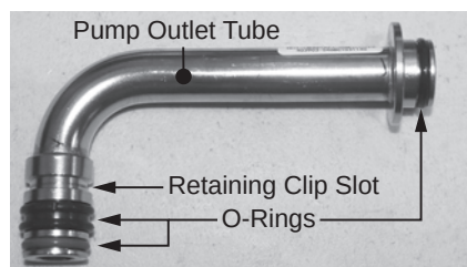
Figure 165 - Pump outlet tube O-rings
