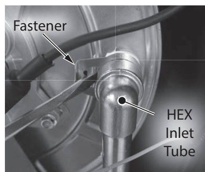
Figure 189 - Remove fastener securing HEX inlet tube
