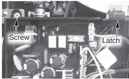
Figure 107 - Control board location
