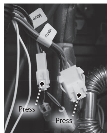
Figure 82 - Locate venturi wire harnesses
