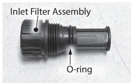
Figure 154 - O-ring location
