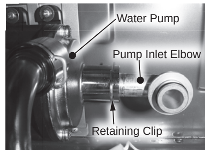
Figure 178 - Pump inlet elbow location
