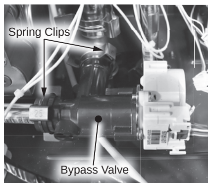
Figure 159 - Bypass valve location
