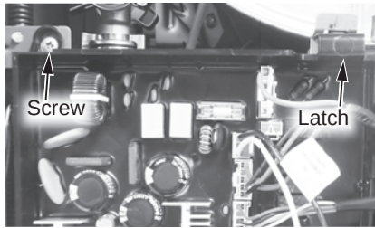
Figure 198 - Control board location
