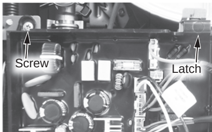
Figure 57 - Control board screw location
