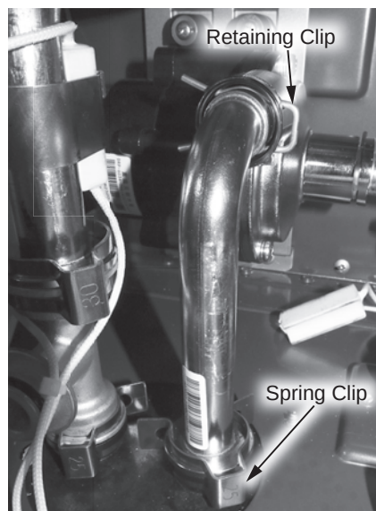
Figure 164 - Pump outlet tube location
