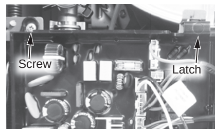
Figure 241 - Control board location
