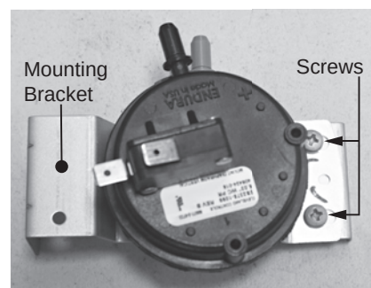
Figure 68 - Pressure switch mounting bracket
