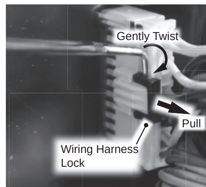
Figure 19 - Black harness lock removal
