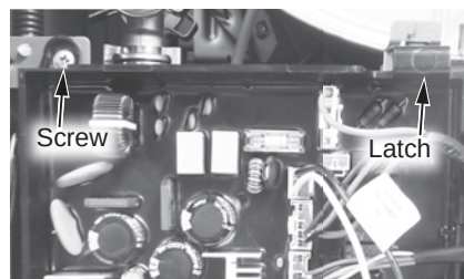
Figure 76 - Control board location
