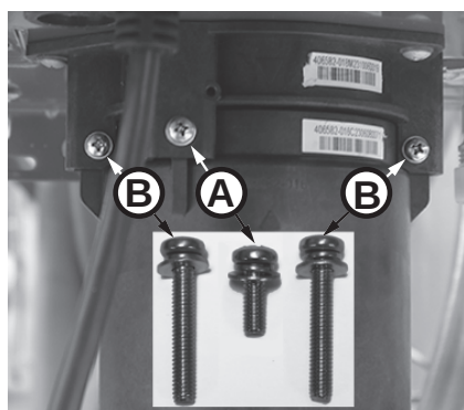
Figure 155 - Identify cartridge screws
