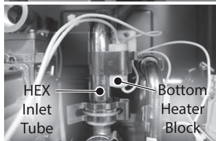
Figure 131 - Remove heater blocks from HEX inlet tube
