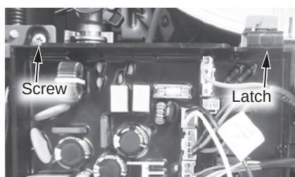
Figure 224 - Control Board screw location
