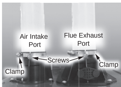
Figure 59 - Flue exhaust port and intake air port location
