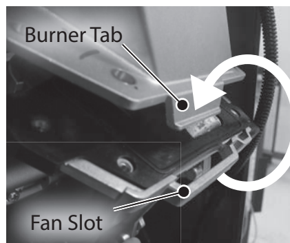
Figure 153 - Burner tab and fan slot
