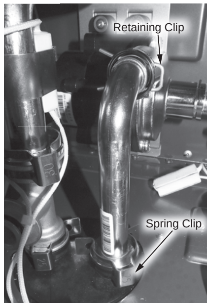
Figure 180 - Pump outlet tube location
