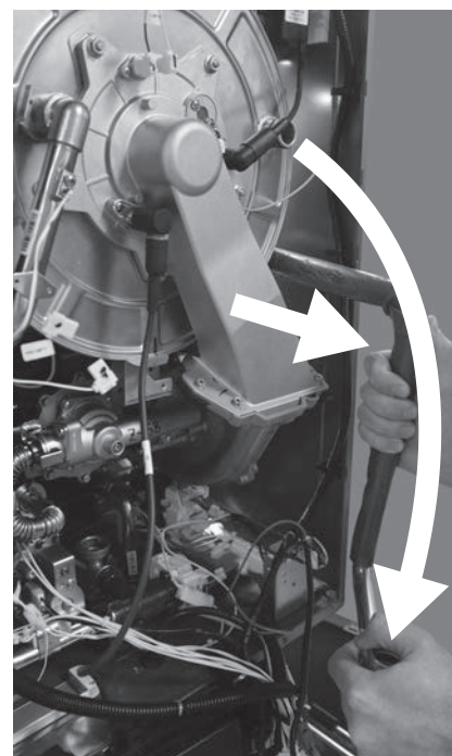
Figure 190 - Lift & pull HEX inlet tube toward you
