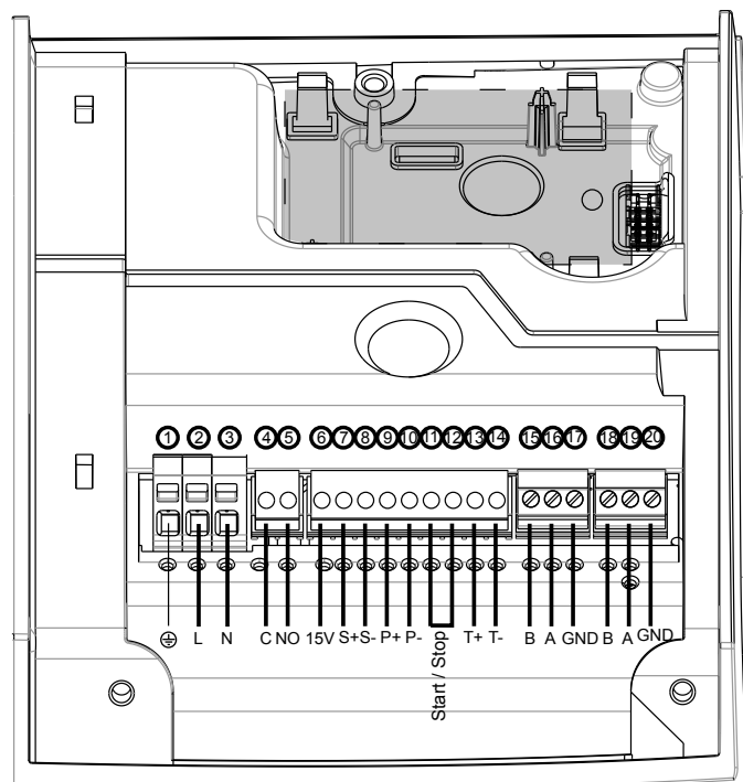
Figure 4: Connection diagram
